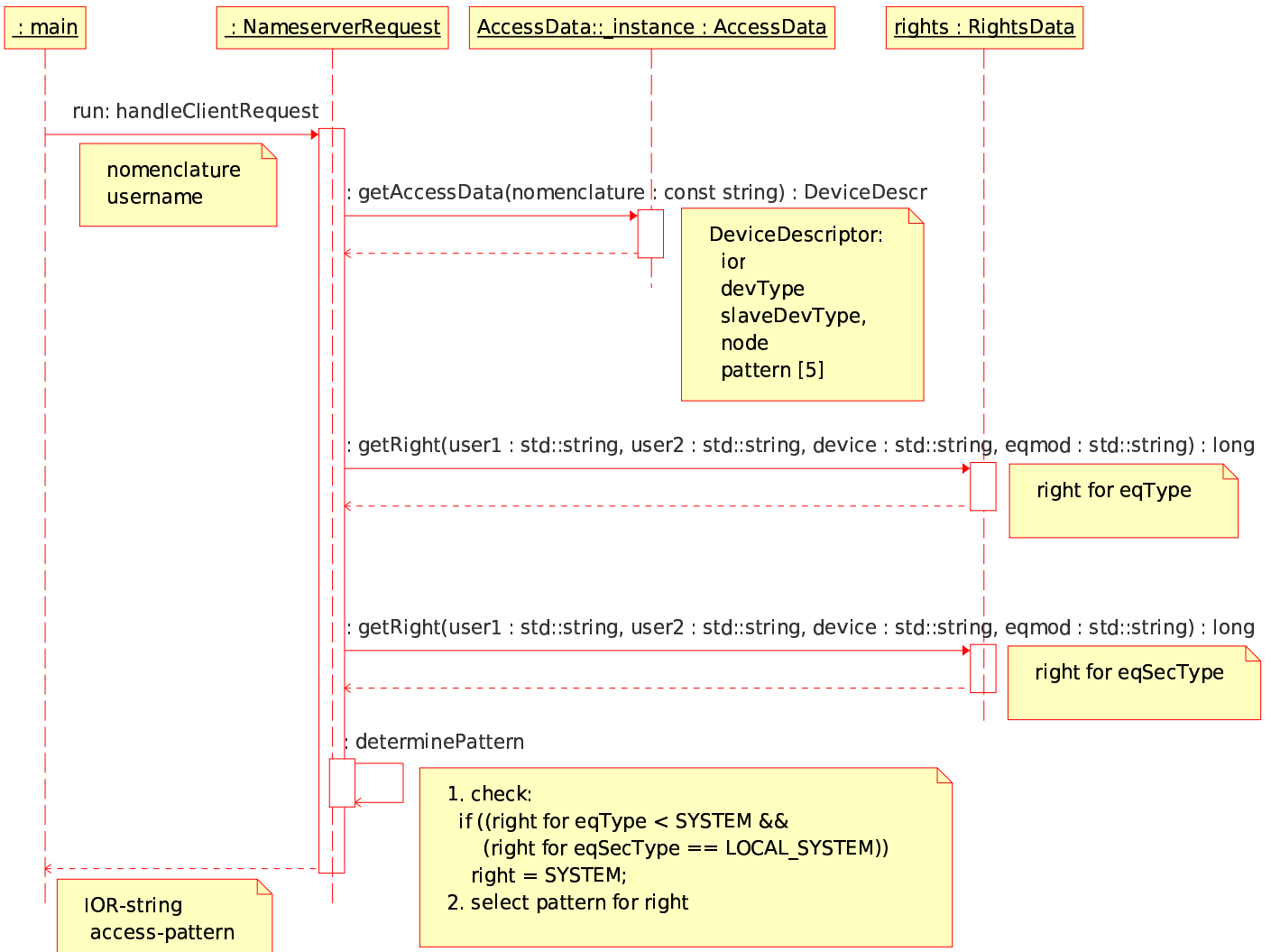
Diagram: AccessRequest Page 1
